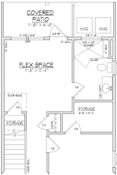
FIRST FLOOR PLAN w/ OPT. FLEX SPACE
