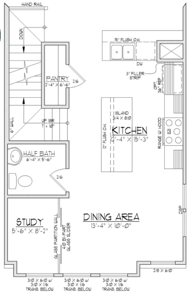
SECOND FLOOR PLAN B w/ OPT. STUDY
