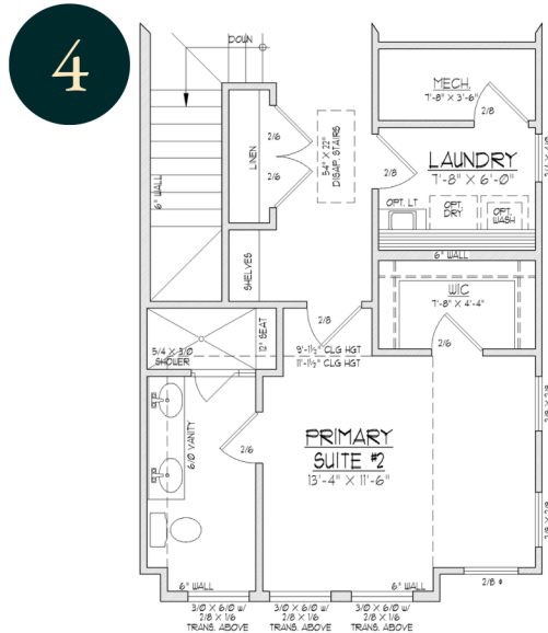
THIRD FLOOR PLAN B w/ OPT. DUAL PRIMARY
