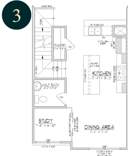
SECOND FLOOR PLAN A w/ OPT. STUDY
