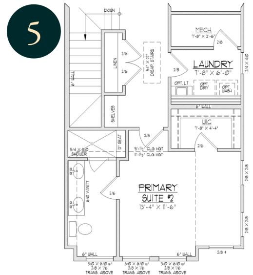
THIRD FLOOR PLAN A w/ OPT. DUAL PRIMARY
