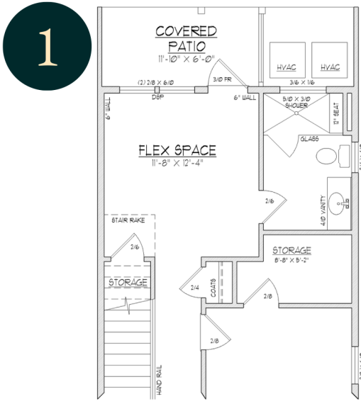
FIRST FLOOR PLAN w/ OPT. FLEX SPACE
