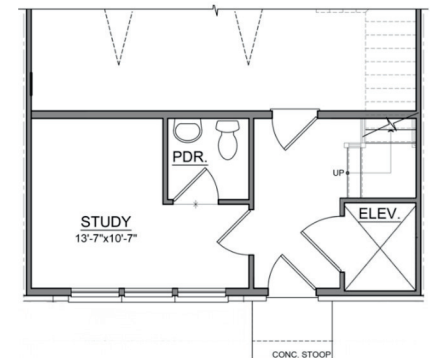
OPT. FIRST FLOOR PLAN STUDY
