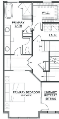
OPT. SECOND FLOOR PLAN DELUXE PRIMARY
