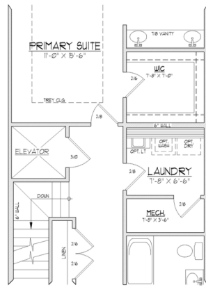
THIRD FLOOR PLAN W/ OPT. ELEVATOR
