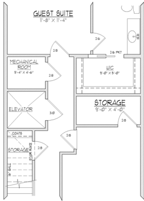
FIRST FLOOR PLAN W/ OPT. ELEVATOR
