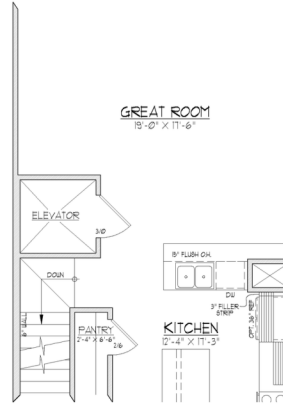
SECOND FLOOR PLAN W/ OPT. ELEVATOR
