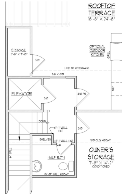
TERRACE FLOOR PLAN w/ OPT. ELEVATOR
