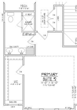
THIRD FLOOR PLAN B w/ OPT. DUAL PRIMARY
