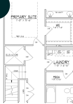
THIRD FLOOR PLAN w/ OPT. ELEVATOR
