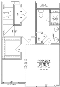
THIRD FLOOR PLAN A w/ OPT. DUAL PRIMARY
