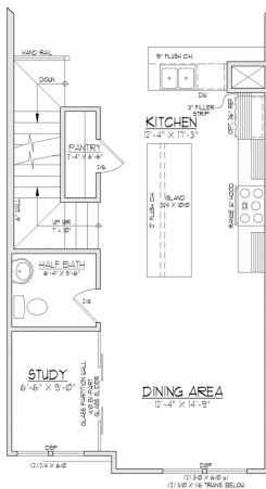
SECOND FLOOR PLAN A w/ OPT. STUDY
