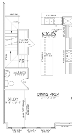
SECOND FLOOR PLAN B w/ OPT. STUDY
