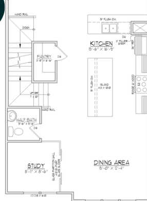
SECOND FLOOR PLAN A w/ OPT. STUDY
