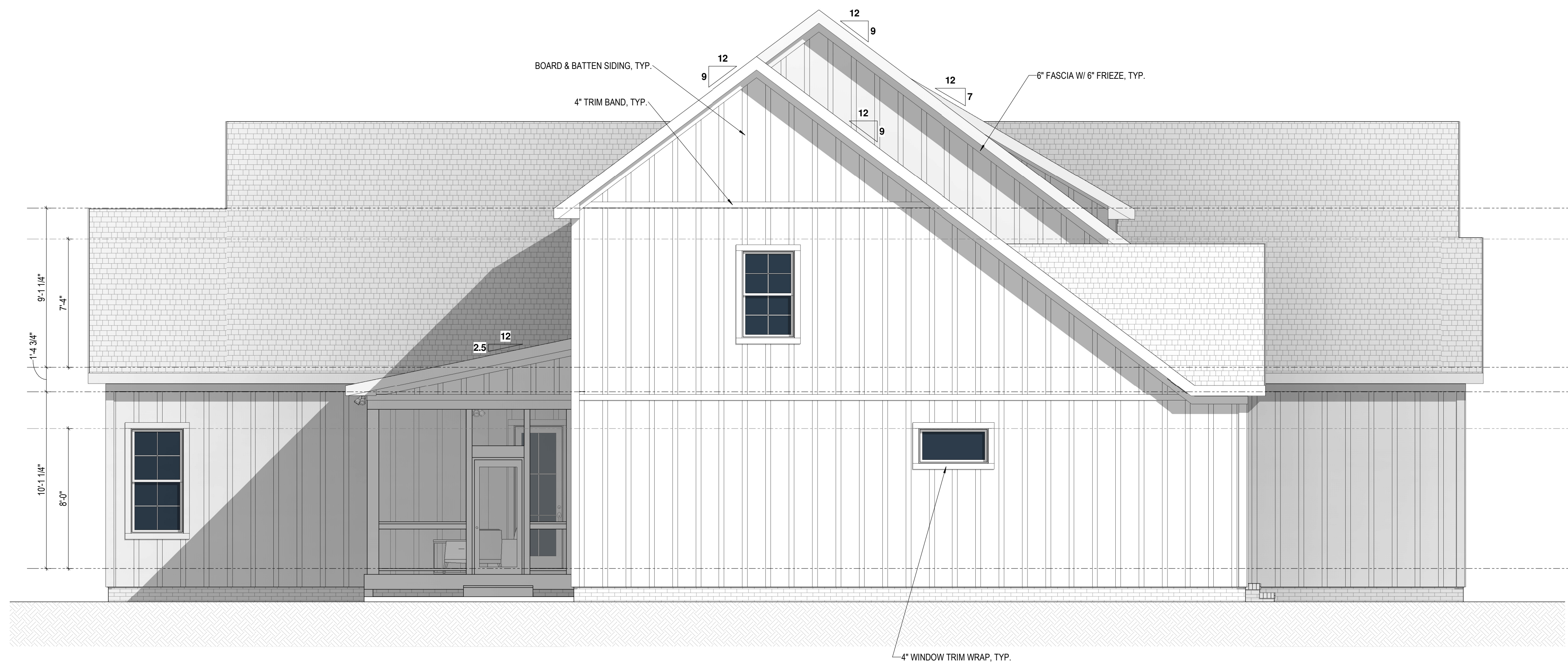
2 LEFT ELEVATION A-1.2 1/4" = 1'-0"
