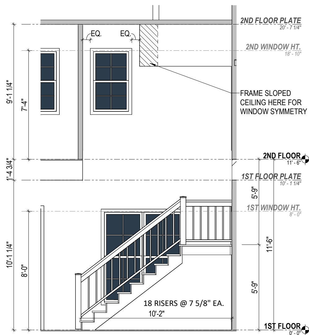
2 Stair Section A-2.3 1/4" = 1'-0"
