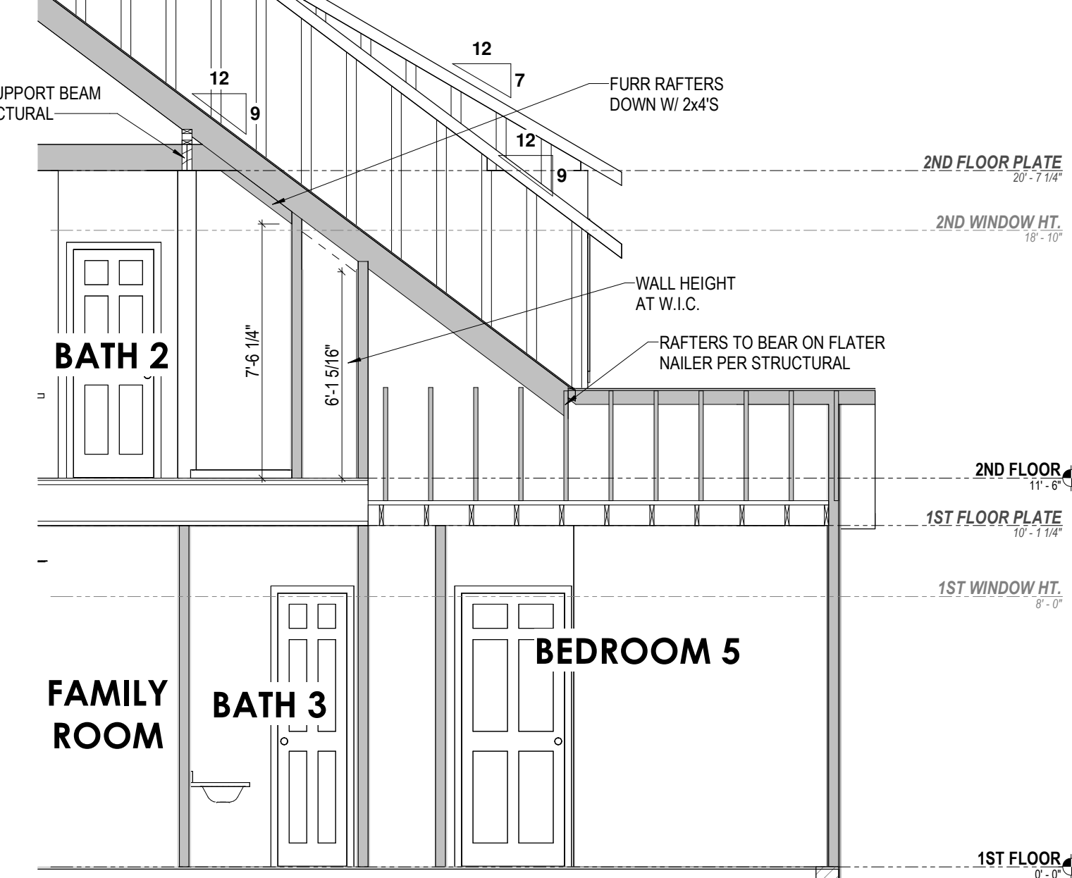
6 Bath 2 Section A-5 1/4" = 1'-0"
