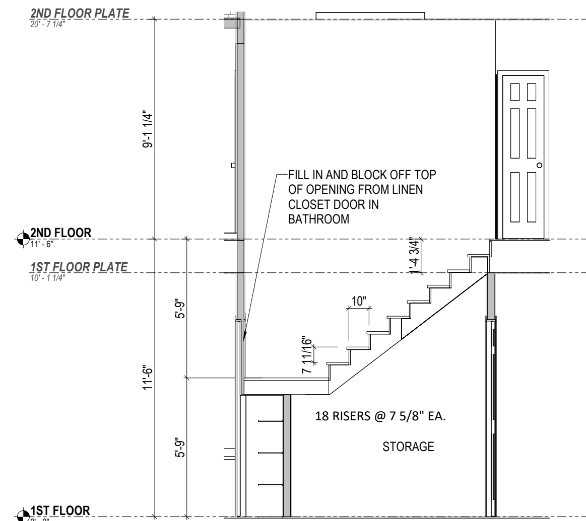
3 Stair Section 2 A-2.3 1/4" = 1'-0"
