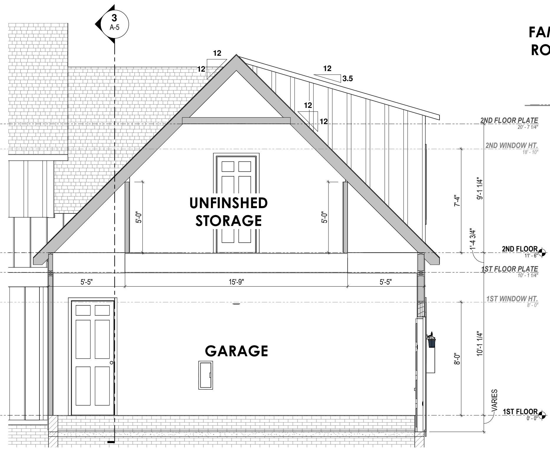
2 Garage Section A-5 1/4" = 1'-0"
