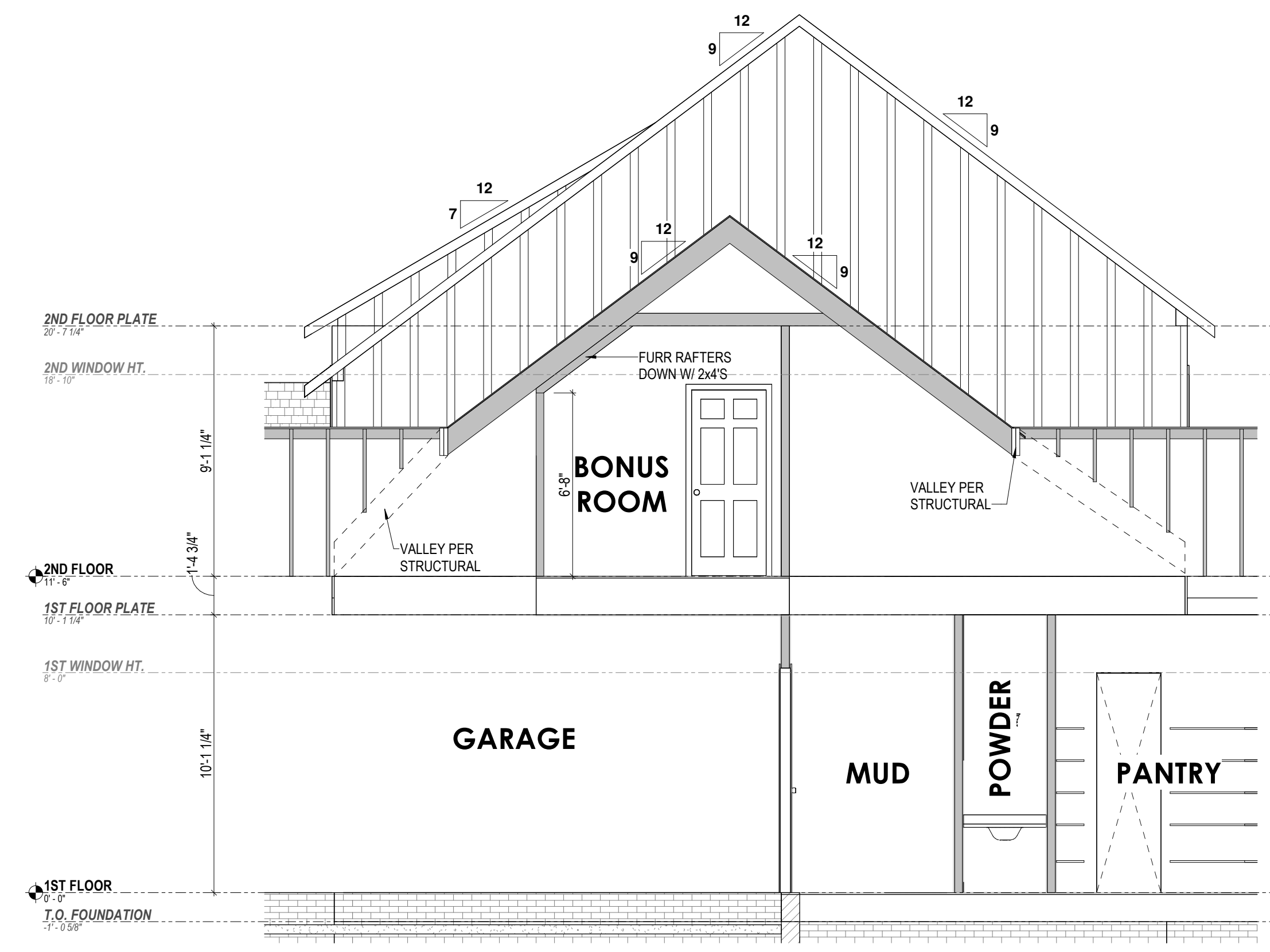
3 Bonus Room Connection Section A-5 1/4" = 1'-0"
