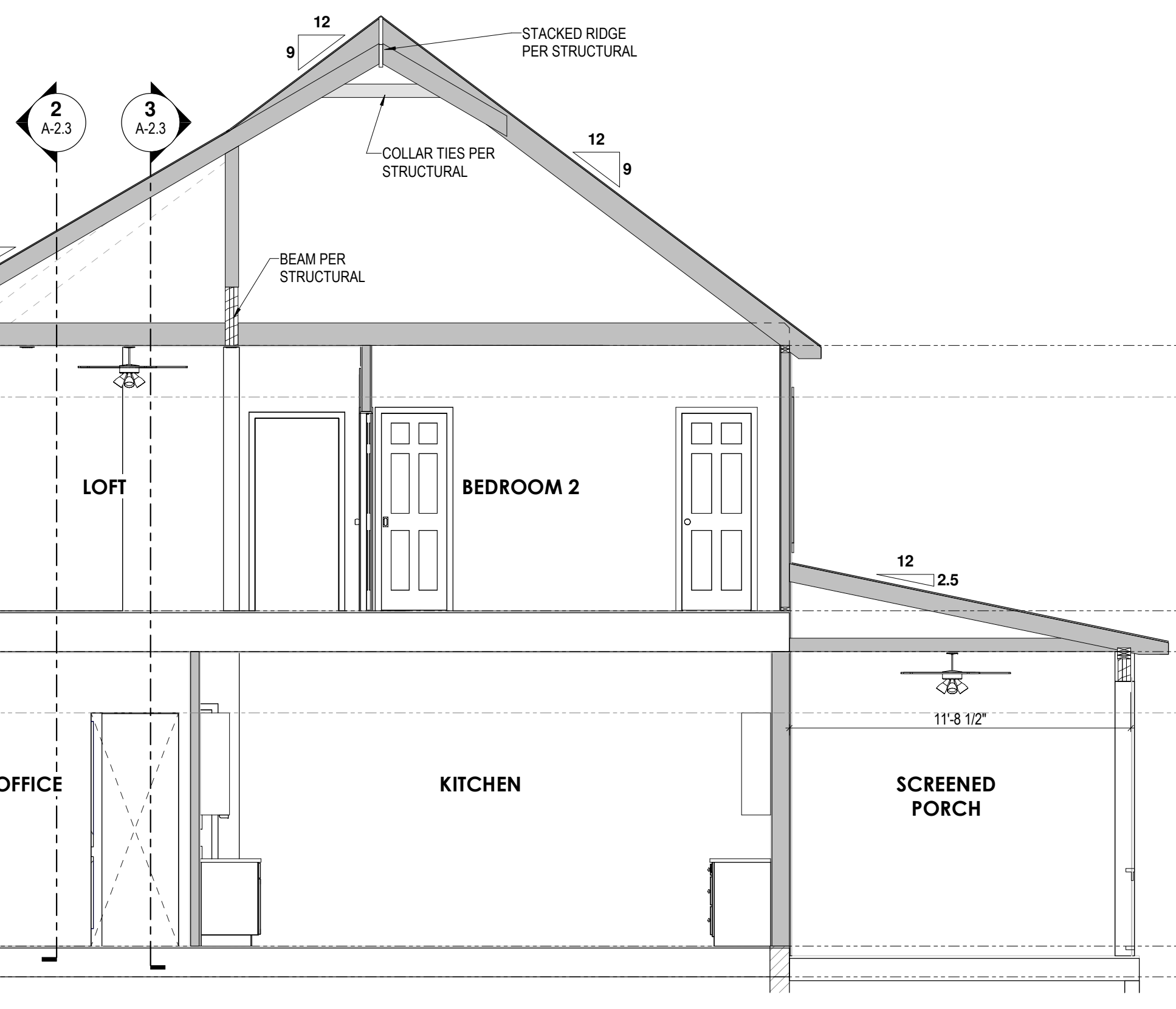
5 Building Section1 A-5 1/4" = 1'-0"
