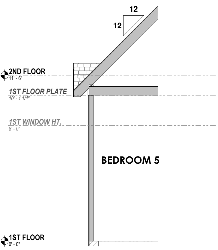
7 Bedroom 5 Section A-5 1/4" = 1'-0"
