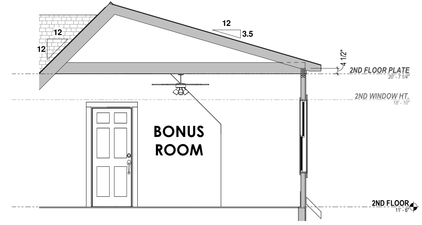
4 Bonus Room Dormer Section A-5 1/4" = 1'-0"
